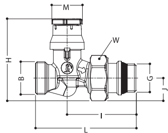
R412TG
