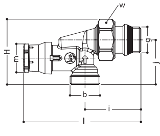
R415TG
