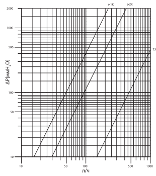
R401H 3/4"
