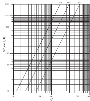
R402H 1/2"
