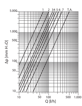
R415PTG
