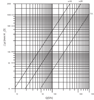
R403H 1/2"
