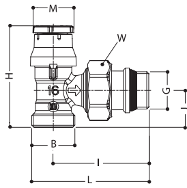
R411TG
