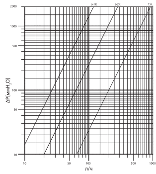
R401H 1/2"
