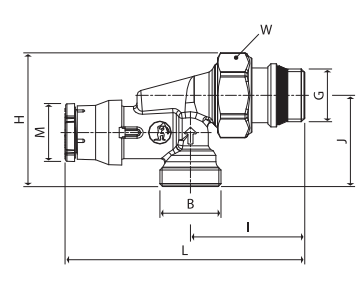
R415PTG
