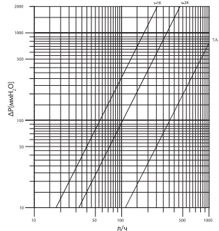
R402H 3/4"
